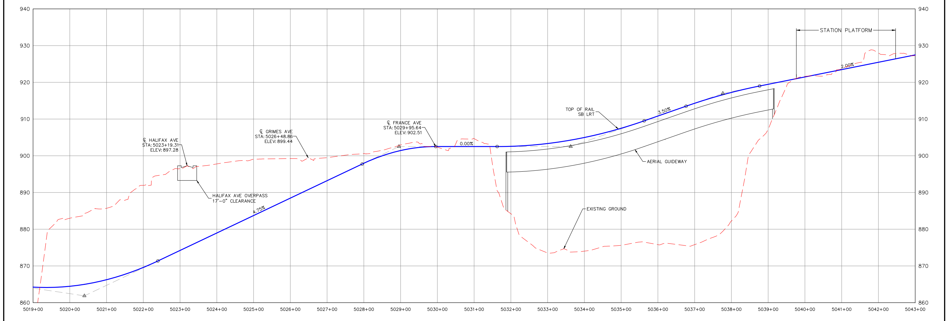
FIGURE 4 - 34TH AVE ALIGNMENT AND PROFILE SHEET 1 OF 2
