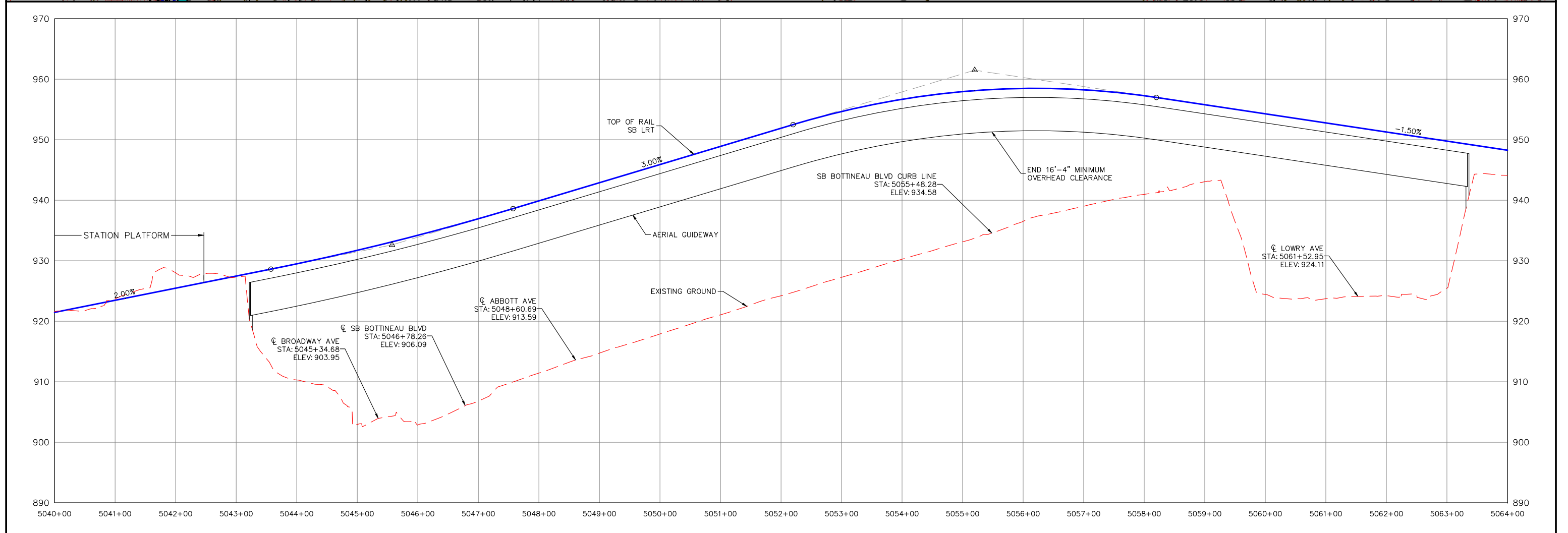
FIGURE 4 - 34TH AVE ALIGNMENT AND PROFILE SHEET 2 OF 2
